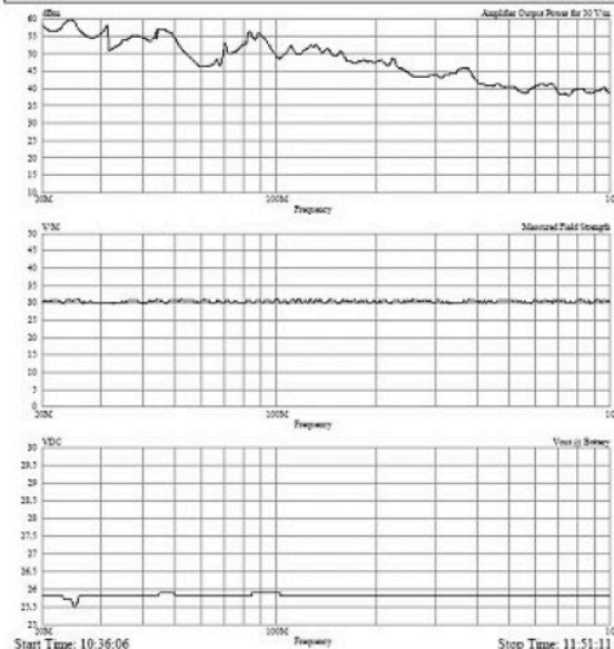
Radiated Immunity Test Data
