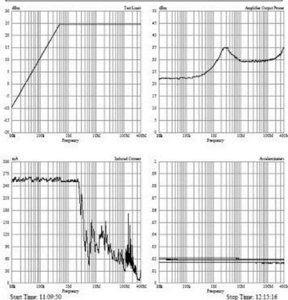
Conducted Immunity Test Data
