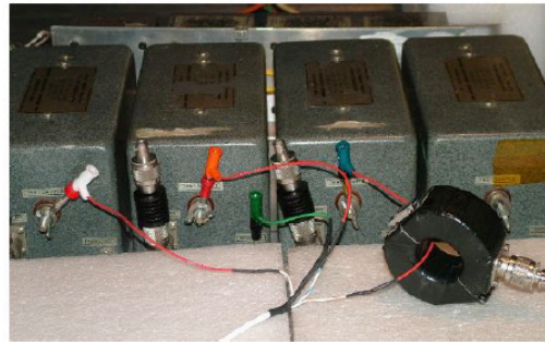
Conducted Emissions Test Setup
