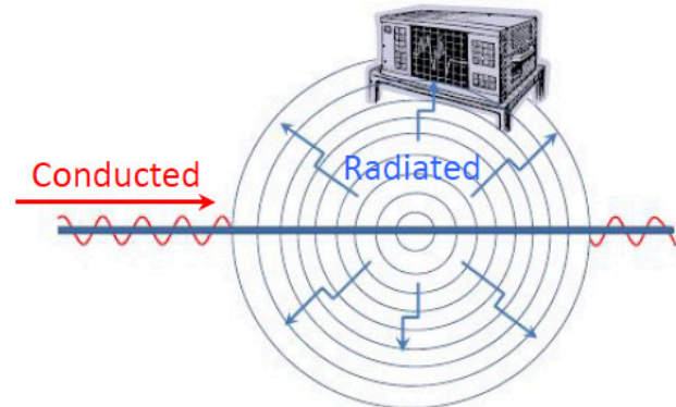
Figure 4 – Conduction → Radiation
